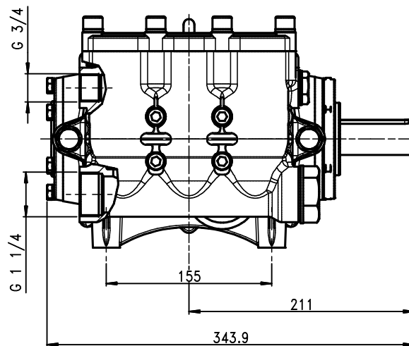
Overall dimensions
